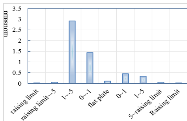
Figure 1. The stocks raising and declining on April 16, 2025. [4]
