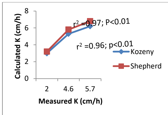
Fig. 1. Relation between calculated and measured hydraulic conductivities
