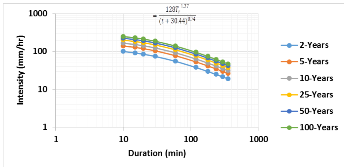
Figure 3.1.: IDF curves by Gumbel method at Umuahia (South-East Nigeria)
