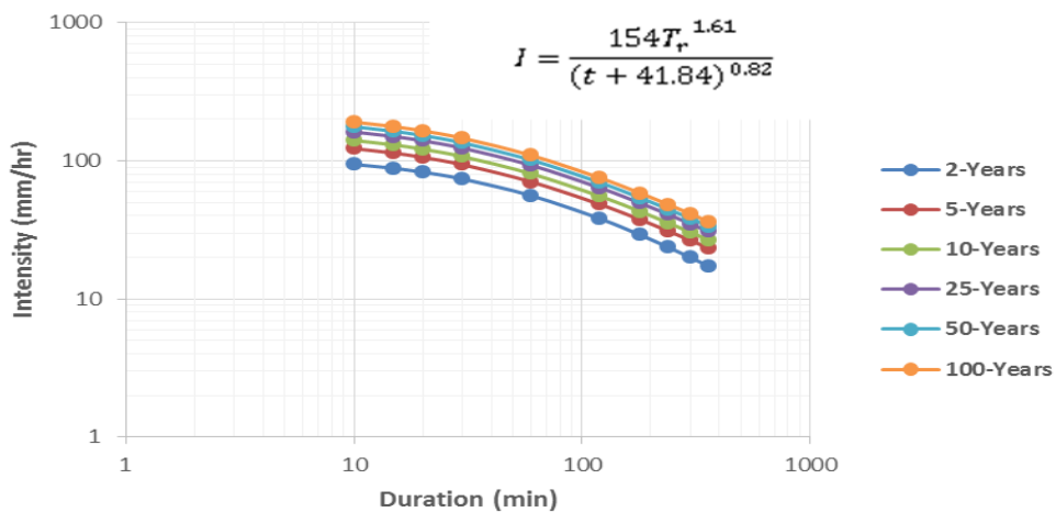
Figure 3.4: IDF curves by LPT III method at Owerri (South-East Nigeria)
