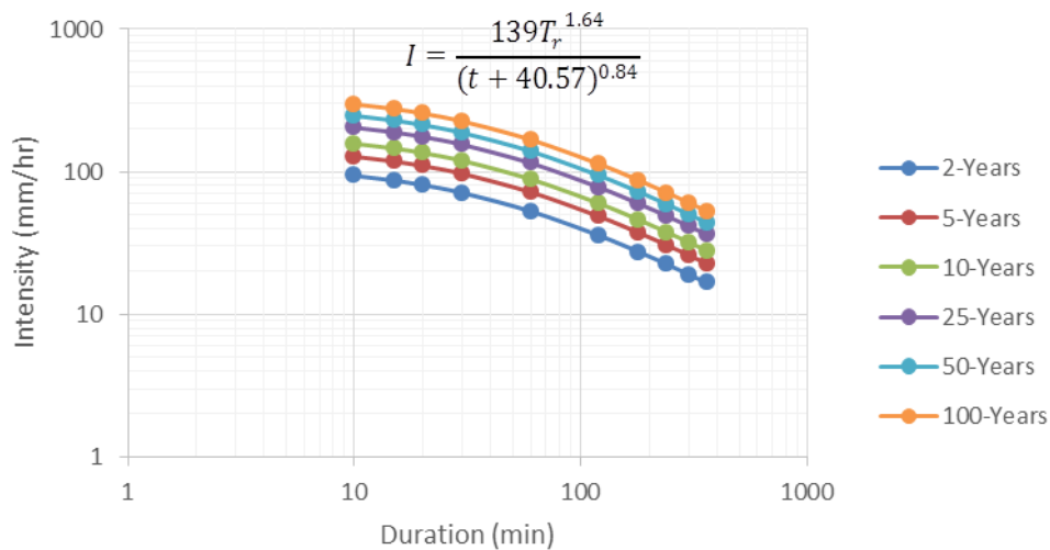
Figure 3.2: IDF curves by LPT III method at Umuahia (South-East Nigeria)
