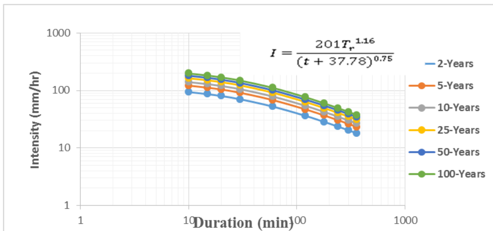
Figure3.3: IDF curves by Gumbel method at Owerri (South-East Nigeria)
