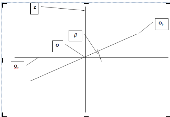
Pic. 1 Cross section of the solar system.
